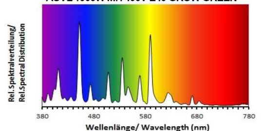
AUVL 1000W MH 400V E40 GROW GREEN
